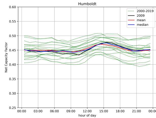
Figure 1. Coos Bay Call Area, Brookings Call Area, and Humboldt Wind Energy Area (WEA) wind rose and potential net capacity factor characteristics
