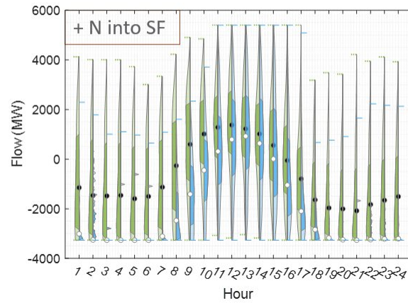
Figure 37. Monthly flow and hourly flow on Path 15 (connecting Southern and Northern California)
