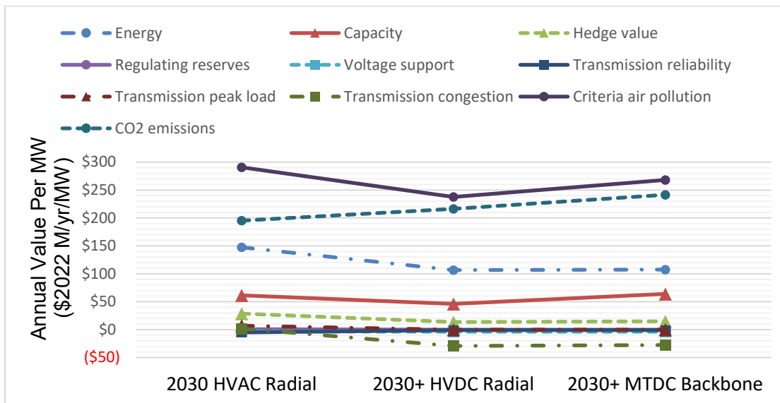
Figure 22. Marginal annual value detail for all topologies
