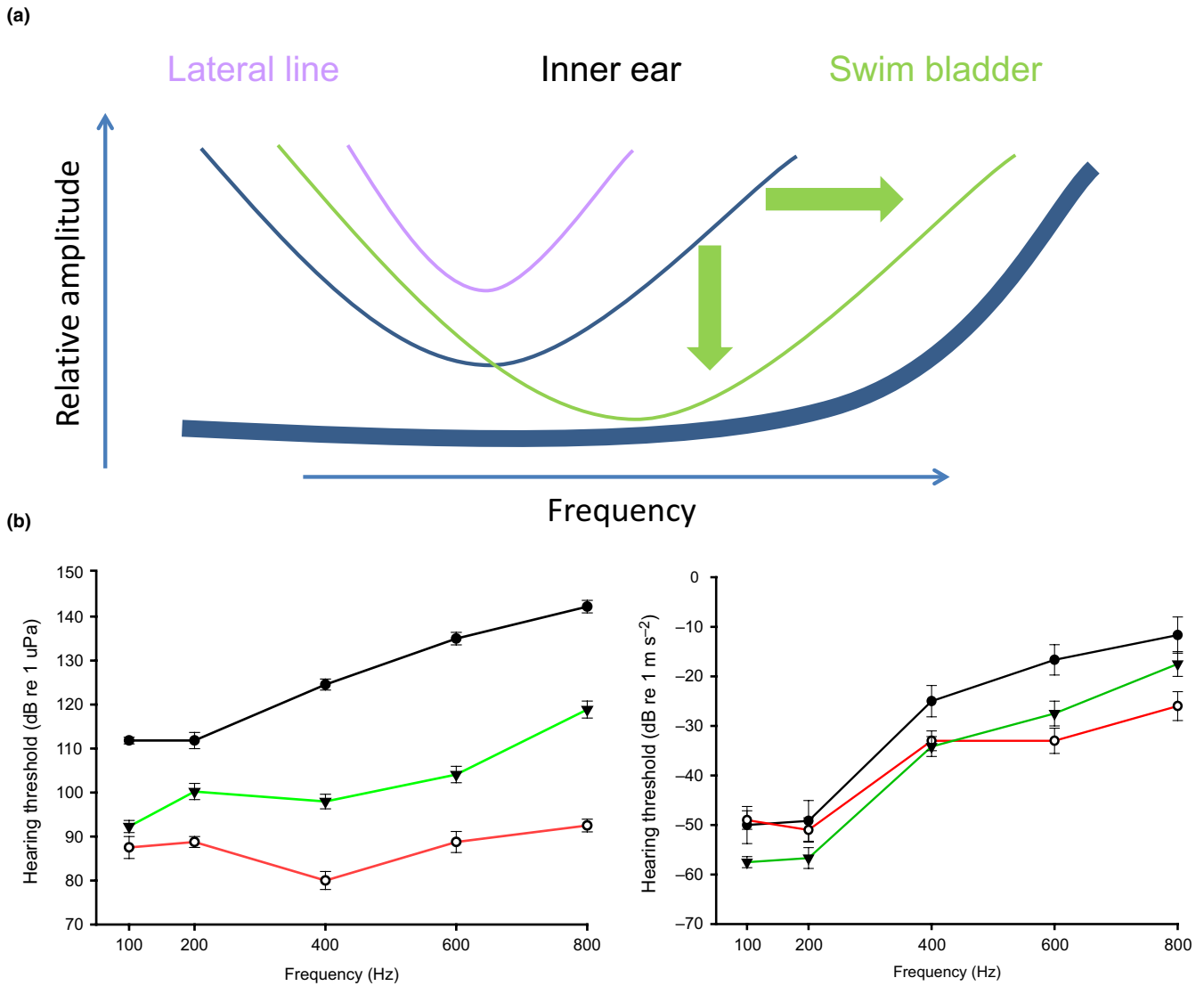
FIGURE 5 (a) Schematic overview of the capability of fish to perceive sounds in terms of relative amplitude and spectrum. The three thin lines reflect the following three auditory pathways: (1) the general sensitivity of all fishes to particle motion through innervation of hair cells close to the otoliths of the inner ear (in dark blue); (2) the sensitivity to particle motion originating from sound pressure through pressure-to-motion transduction for fish species with a swim bladder (in green), which typically results in a lower overall threshold and an extension of sensitivity towards higher frequencies (green arrows); and (3) the sensitivity to particle motion via the lateral line (in lilac). This concerns relatively low frequencies in the flow of water directly surrounding the fish (through movements of the fish itself, water flow currents, or turbulence by other fish or objects) and which is not likely to outcompete the inner ear in sensitivity. The bold blue line represents the cumulative shape of the audiogram: the sensitivity to sound across frequencies, attributable to a variable and unquantified combination of sensitivity through the three pathways. (b) Hearing thresholds of three different species for independent assessments of sound pressure level (left) and sound particle acceleration level (right). The common triplefin ( Forsterygion lapillum , Tripterygiidae) has no swim bladder (black lines). The New Zealand bigeye ( Pempheris adspersus , Pempheridae) has a swim bladder but no Weberian ossicles (green lines). The goldfish ( Carassius auratus , Cyprinidae) has a swim bladder and specialized conduction to the inner ear via Weberian ossicles (red lines). In terms of particle motion, all three fish species have similar hearing thresholds, but when expressed as pressure thresholds, the goldfish is the most sensitive, followed by the bigeye and the triplefin being the least sensitive (Radford et al., 2012) [Colour figure can be viewed at wileyonlinelibrary.com ]
