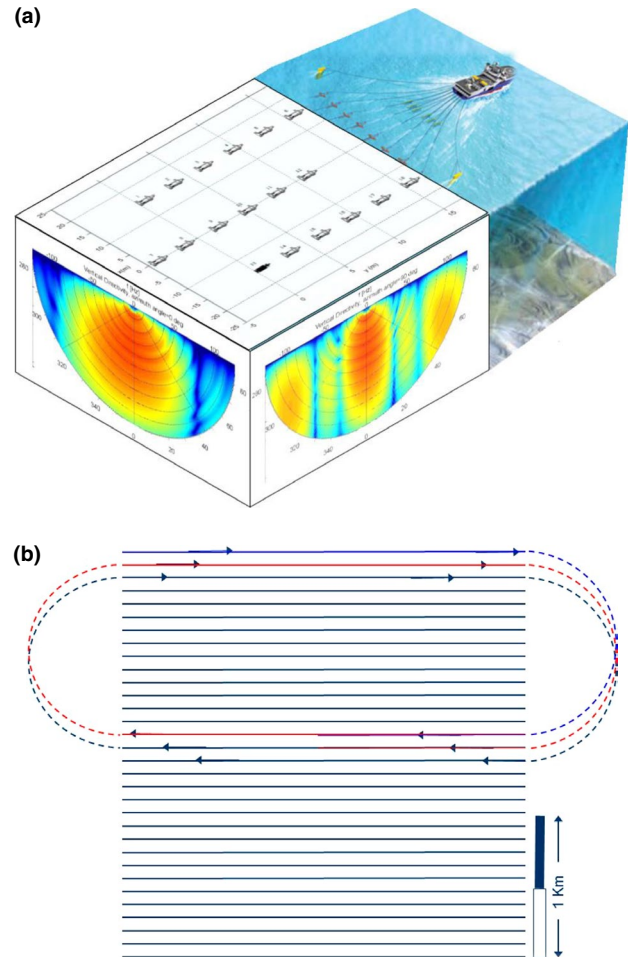
FIGURE 3 (a) Artistic impression of a seismic survey presented with the vertical directivity pattern of the energy source spectral density level (dB re 1\mu\text{Pa}^2 \text{m}^2 \text{s}/\text{Hz} ) for the airgun array at different azimuth angles (courtesy: Özkan Sertlek). We developed an algorithm for the calculation of airgun signatures (AGORA) based on various branches of physics such as bubble motion, gas pressure laws, thermodynamics and mass transfer (Sertlek & Ainslie, 2015), which is now freely available from Leiden University at http://oalib.hlsresearch.com/wileyonlinelibrary.com . (b) Schematic representation of a 3D survey vessel course pattern. Each line represents a vessel sail-line. The arrows indicate vessel direction and pathway, starting in blue, changing to red and grey-blue with time in subsequent tracking courses (courtesy: J. Caldwell, OYO Geospace; and C. Walker, Seabed Geosolutions) [Colour figure can be viewed at wileyonlinelibrary.com ]
